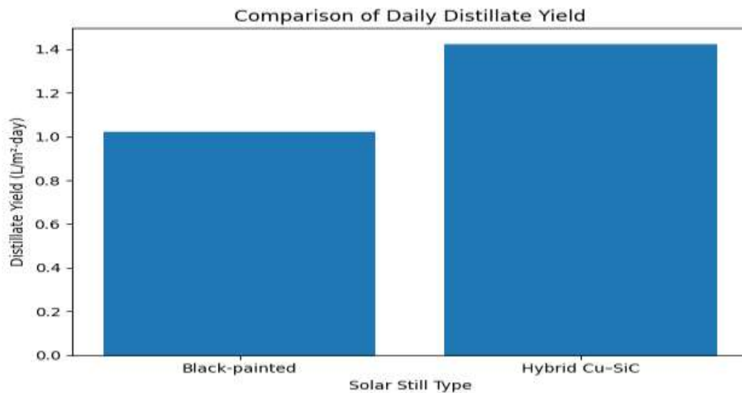
Figure 2. Comparison of daily distillate yield between black - painted and hybrid Cu–SiC solar stills.
